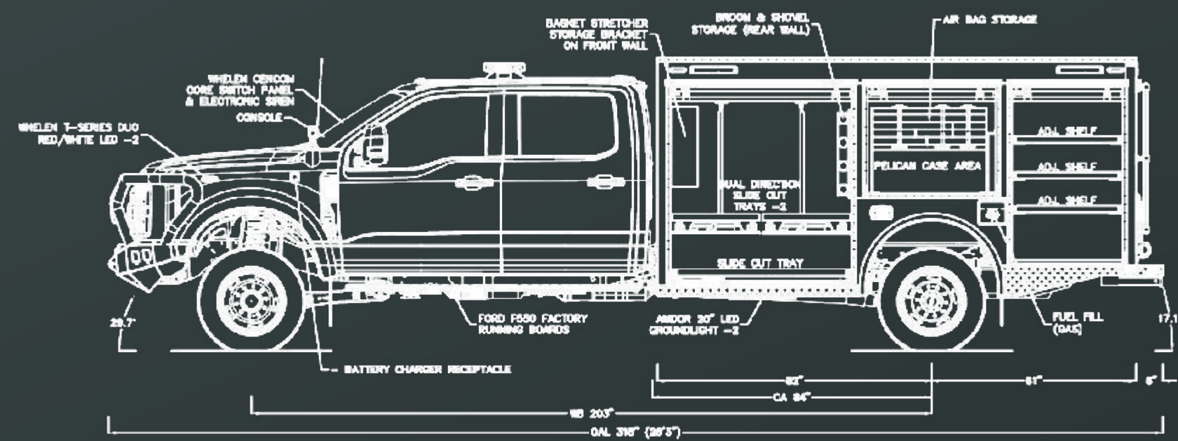
DRIVER SIDE ELEVATION
